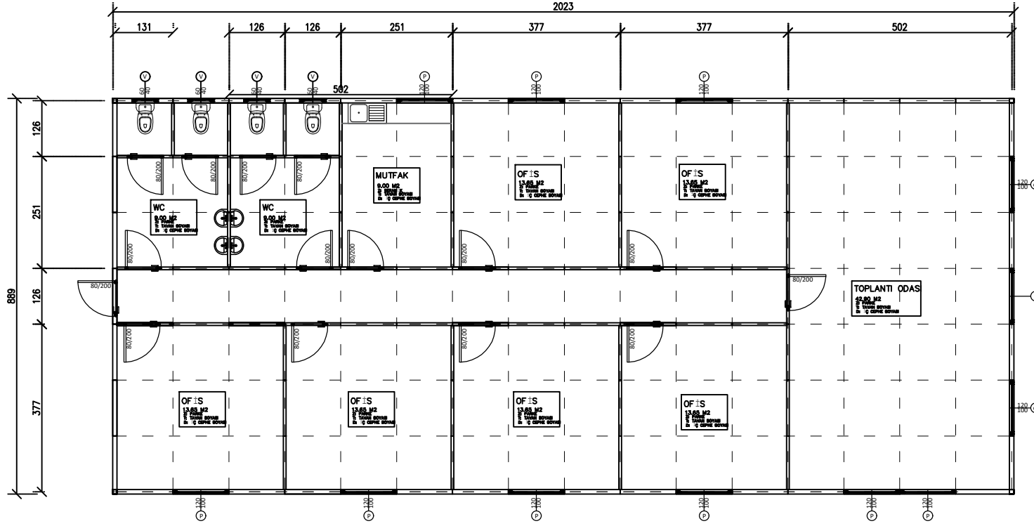
ZEMİN KAT PLANI 180 M2
