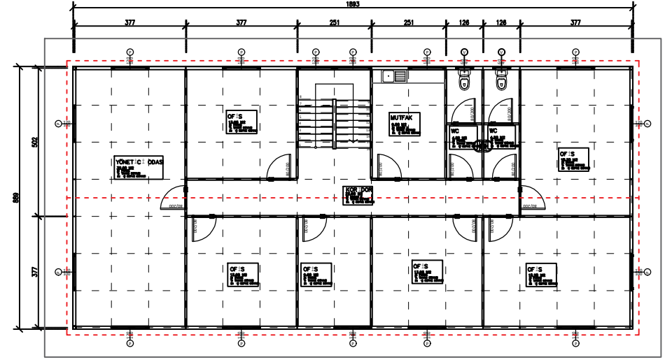
ZEMİN KAT PLANI 168 M2
