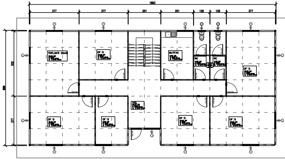
ZEMİN KAT PLANI 165 M2
