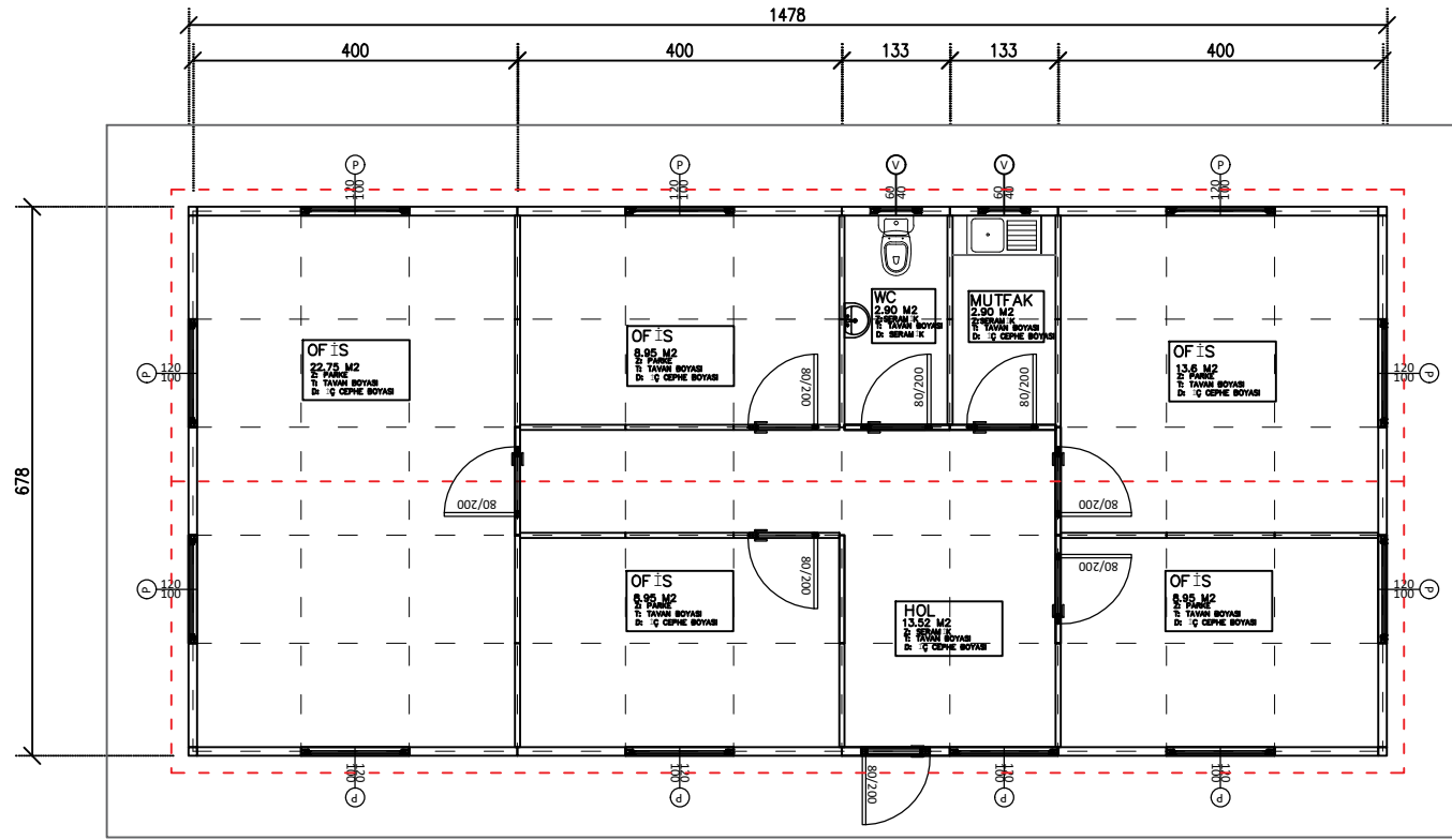
ZEMİN KAT PLANI 89 M2
