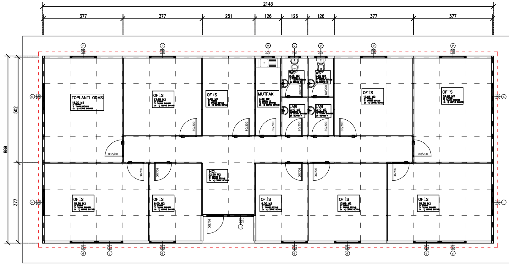
ZEMİN KAT PLANI 190 M2
