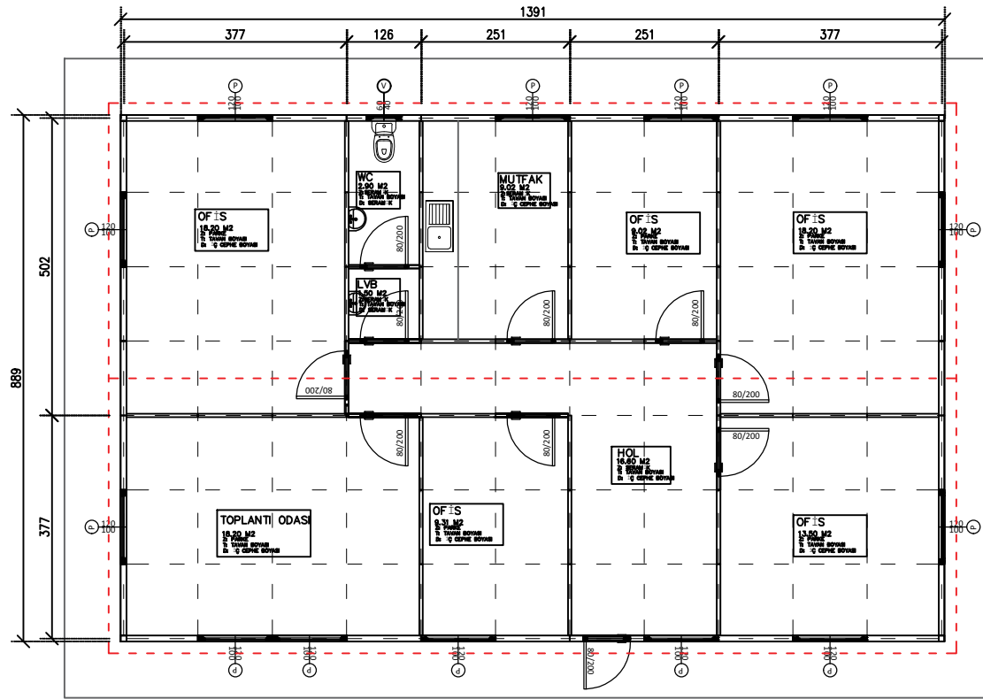
ZEMİN KAT PLANI 123 M2
