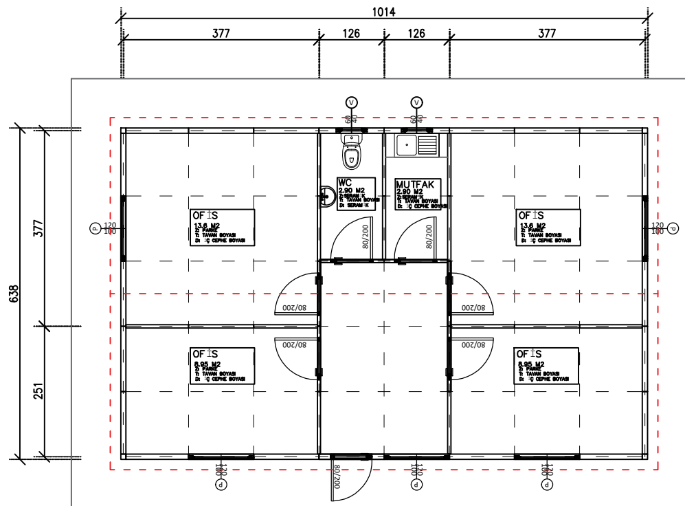
ZEMİN KAT PLANI 65 M2
