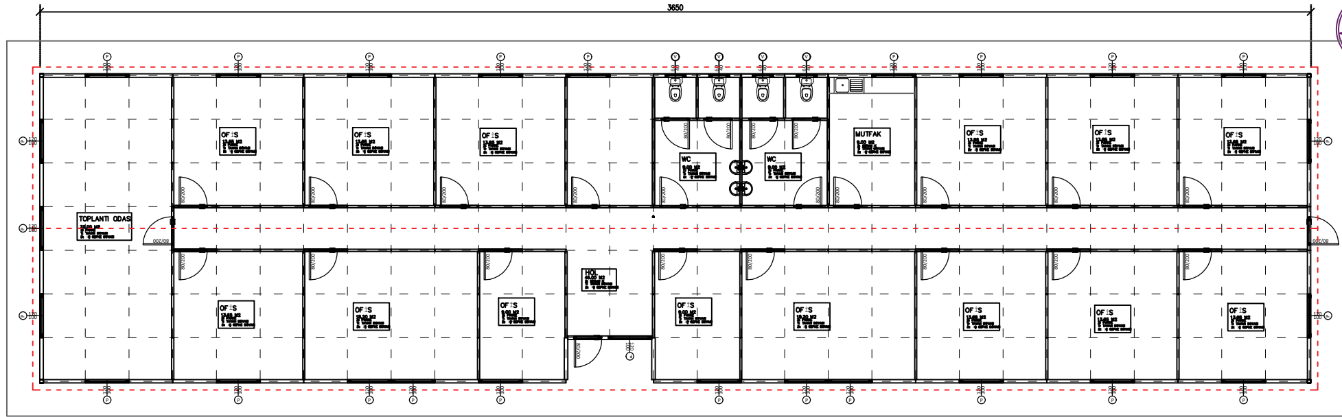
ZEMİN KAT PLANI 324 M2
