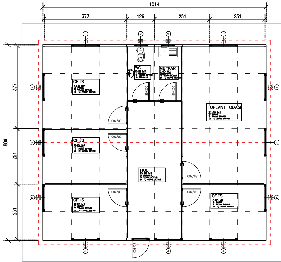
ZEMİN KAT PLANI 90 M2
